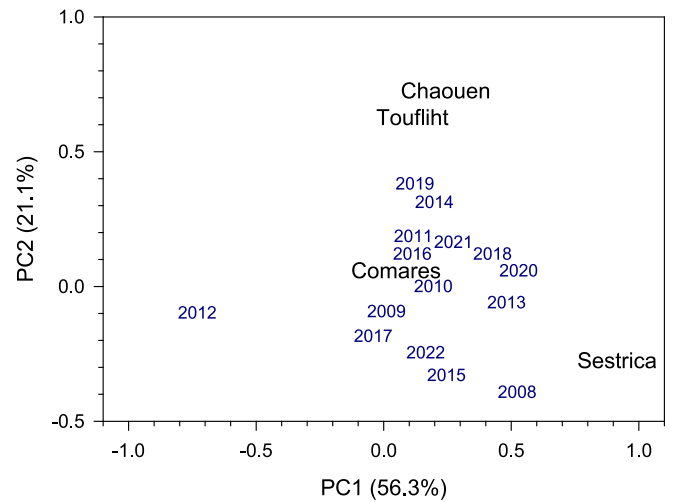
Fig. 3. Biplot showing the scores of the first (PC1) and second (PC2) principal components. Black symbols show the four study sites and blue symbols show the year of cork-ring width indices. The percentage of variance explained by each component is shown between parentheses.
